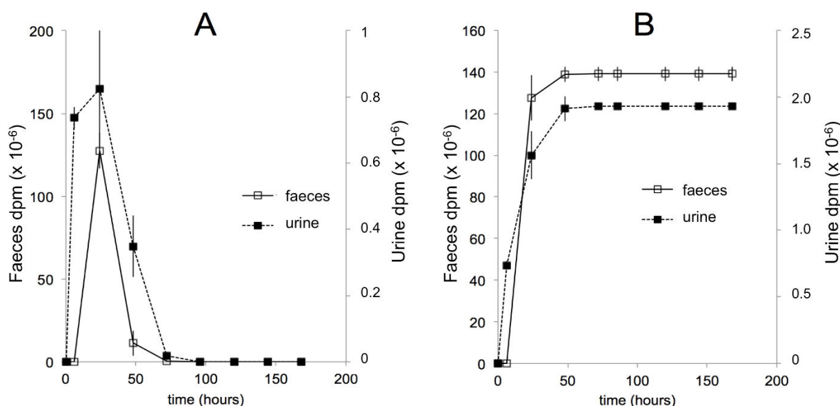
Figure 8. Comparison of the temporal (A) and cumulative (B) urinary and fecal elimination of radioactivity after the oral application of [5,7,9- ^3 H]20E to 6–7 week-old male Wistar rats. After oral application of [ ^3 H]20E, elimination of radioactively labelled 20E and its metabolites is completed within 48 h. The amount of radioactivity recovered from the feces is by far the major route of excretion, since the amount in the urine corresponds to only 1.40% of the total radioactivity recovered. (Reproduced, with permission, from [127]).
